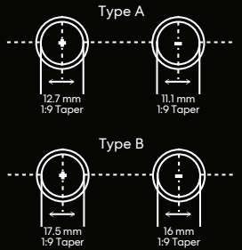
Terminal Types
